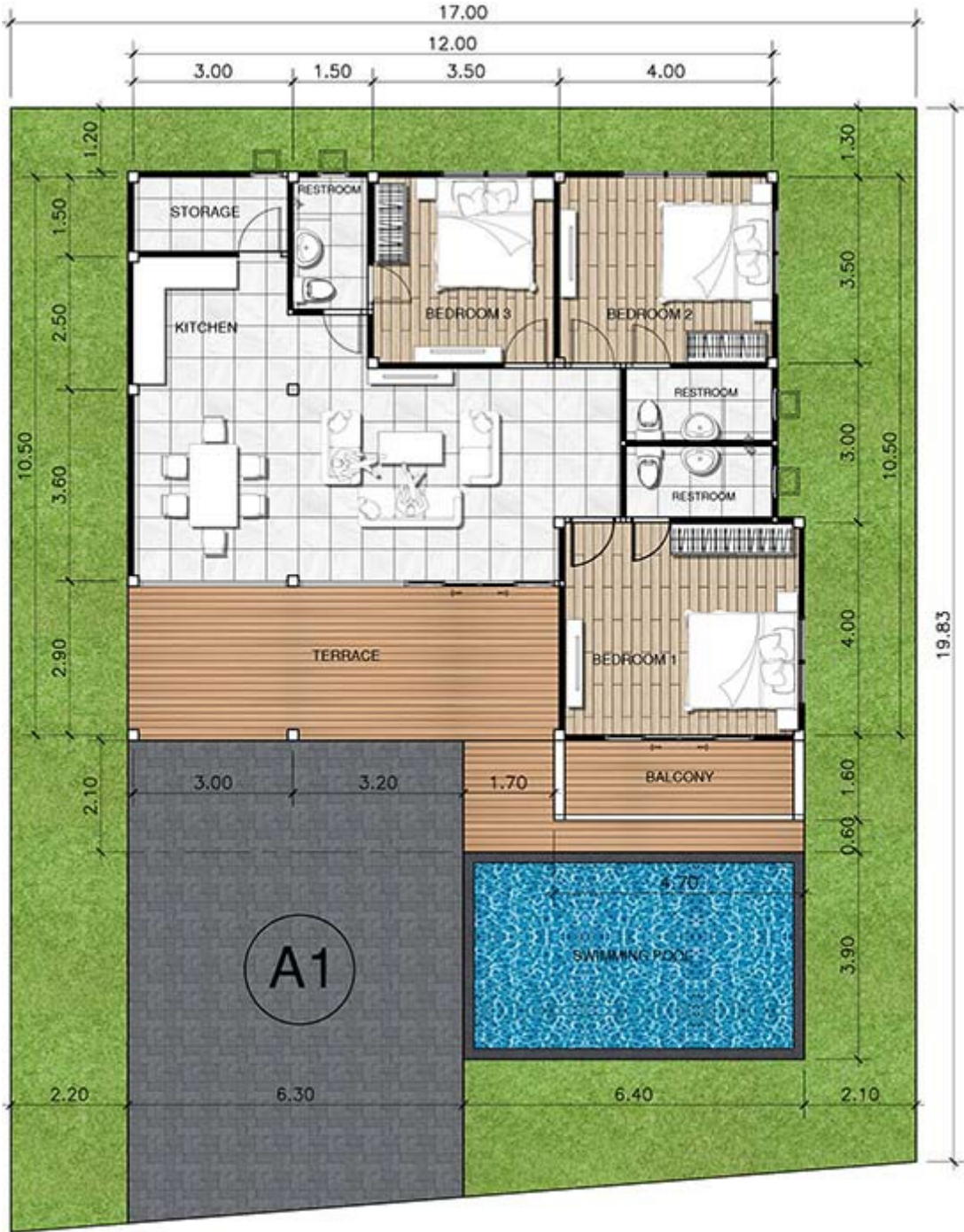
Floor Plan Indigo Residence Sample of House
